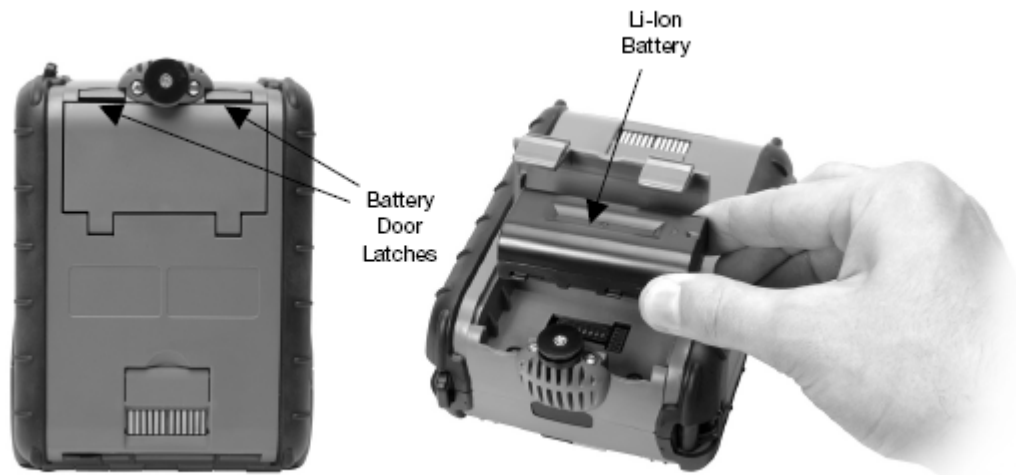
FIGURE 2: INSTALLING THE BATTERY CARTRIDGE
