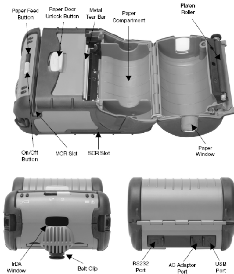
FIGURE 1: PRINTER OVERVIEW
