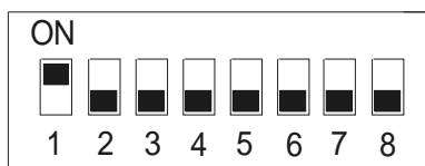
FIGURE 12: EXAMPLE: DIP SWITCH #1 SHOWN IN 'ON' POSITION
