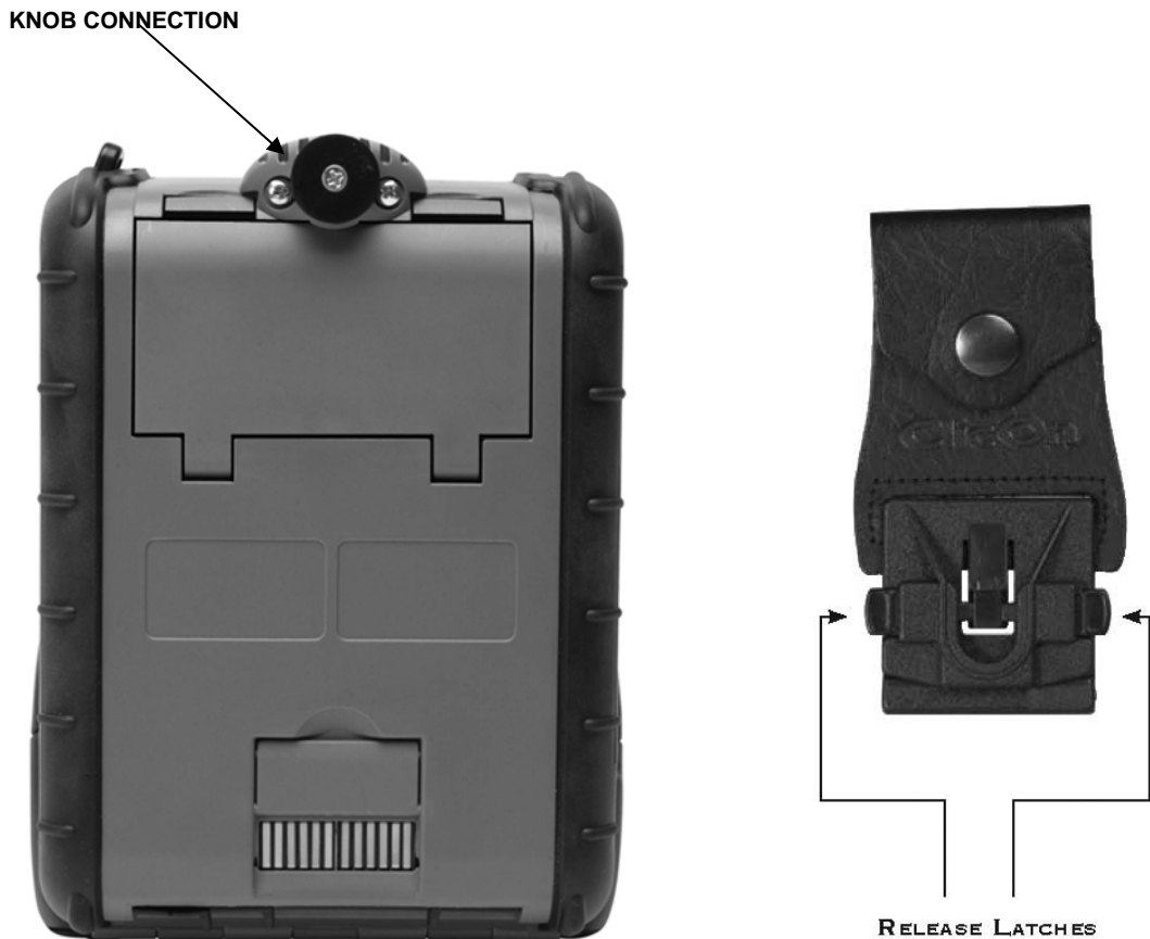
FIGURE 5– KNOB CONNECTION AND QUICK CLIP
