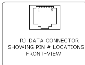
FIGURE 13 – RJ DATA CONNECTOR
