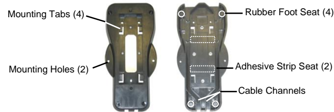
Figure 3 - Horizontal Base Front and Bottom View
