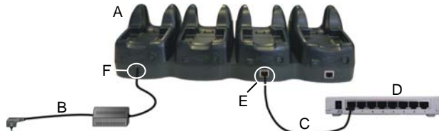
Figure 6 - Ethernet Connection
