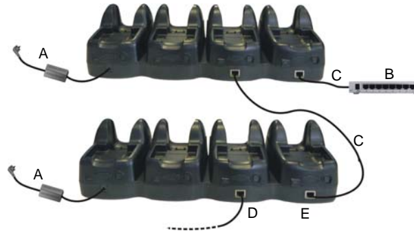
Figure 7 - Daisy chaining Ethernet Connection
